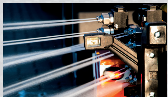
Long throw nozzles up to 15 m over the centre
